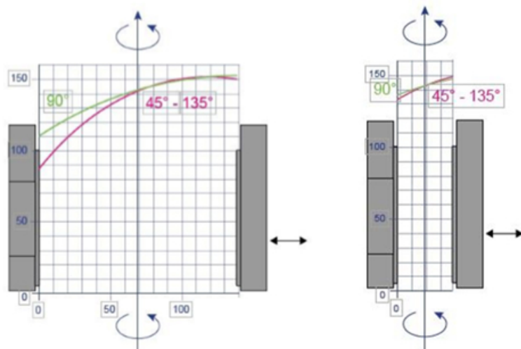
Zaagdiagram Pertici Scarabeo SC 55
